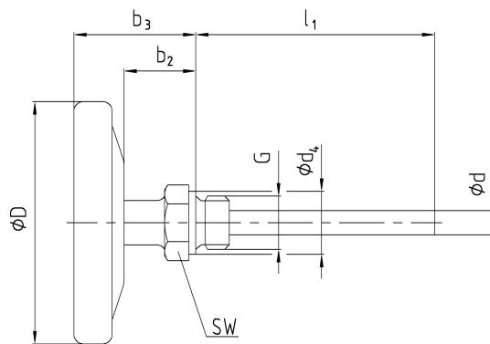
Design for temperatures above 300°C (with spacer b2 = 30mm)
